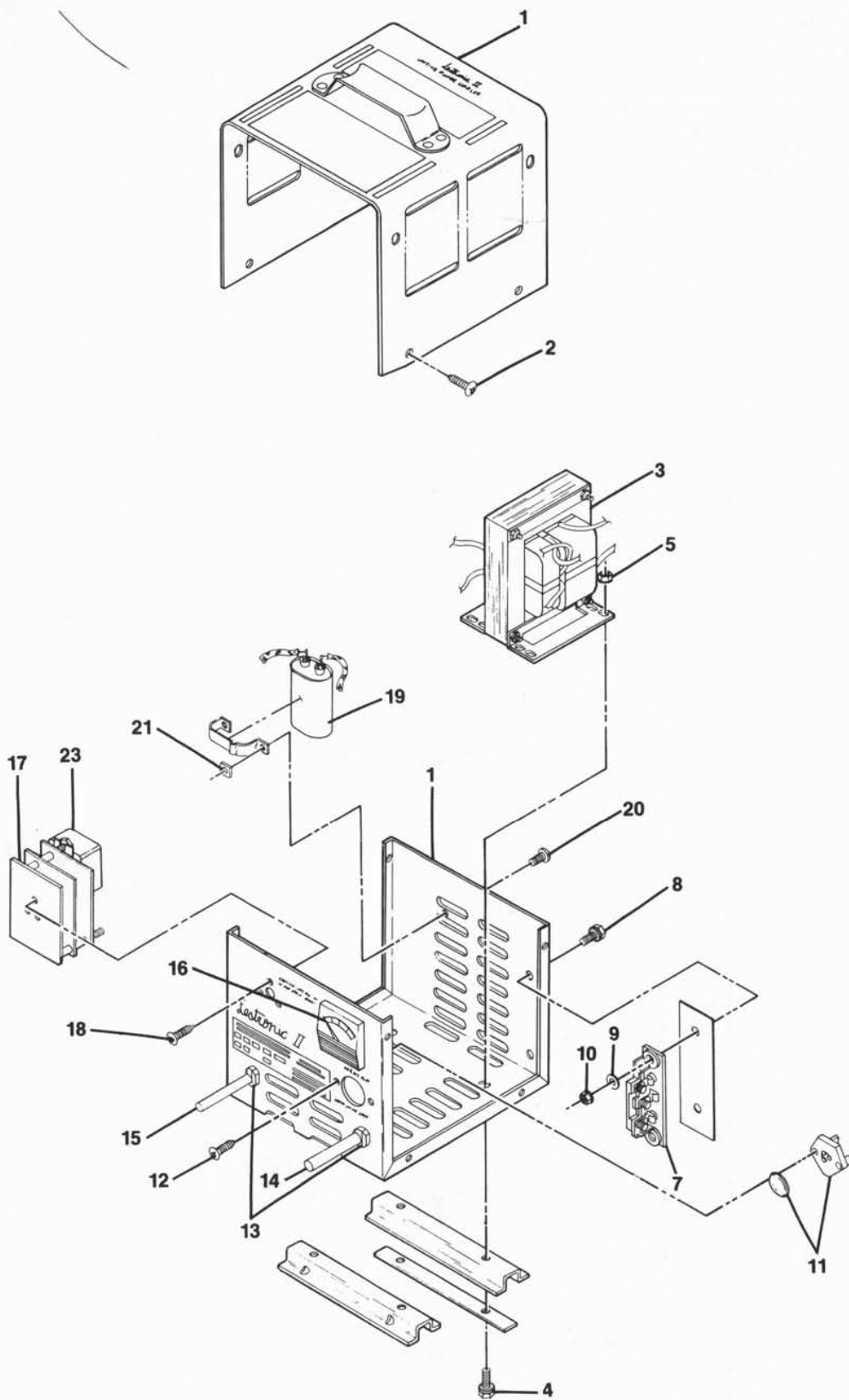
FIGURE 6-2. LESTER BATTERY CHARGER MODEL NO. 7850. SEE LIST 6-2.
